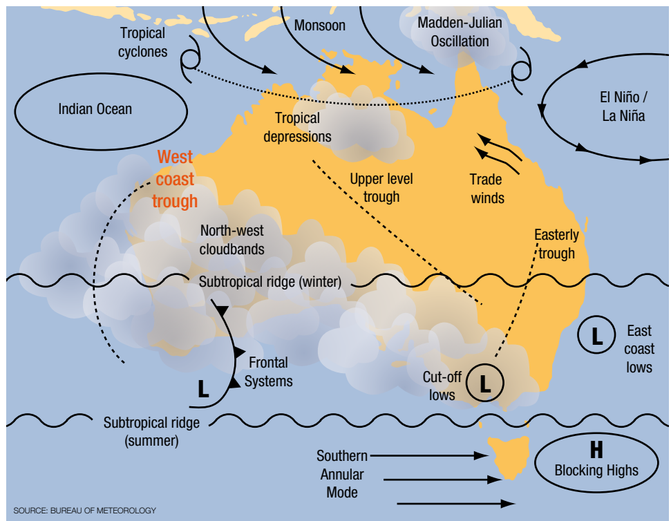
The main influences on Australia's climate. Influences have varying impact in different regions and at different times of year. Visit the 'Our Weather & Climate' page at www.bom.gov.au/wat/ for more information.
