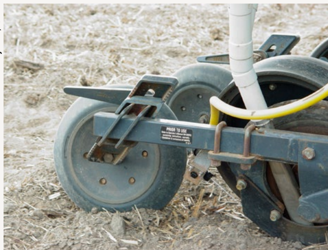
FIGURE 2-13 (a). Spray line attached behind planting tyne/boot used to disperse inoculants into furrow (water injection).
