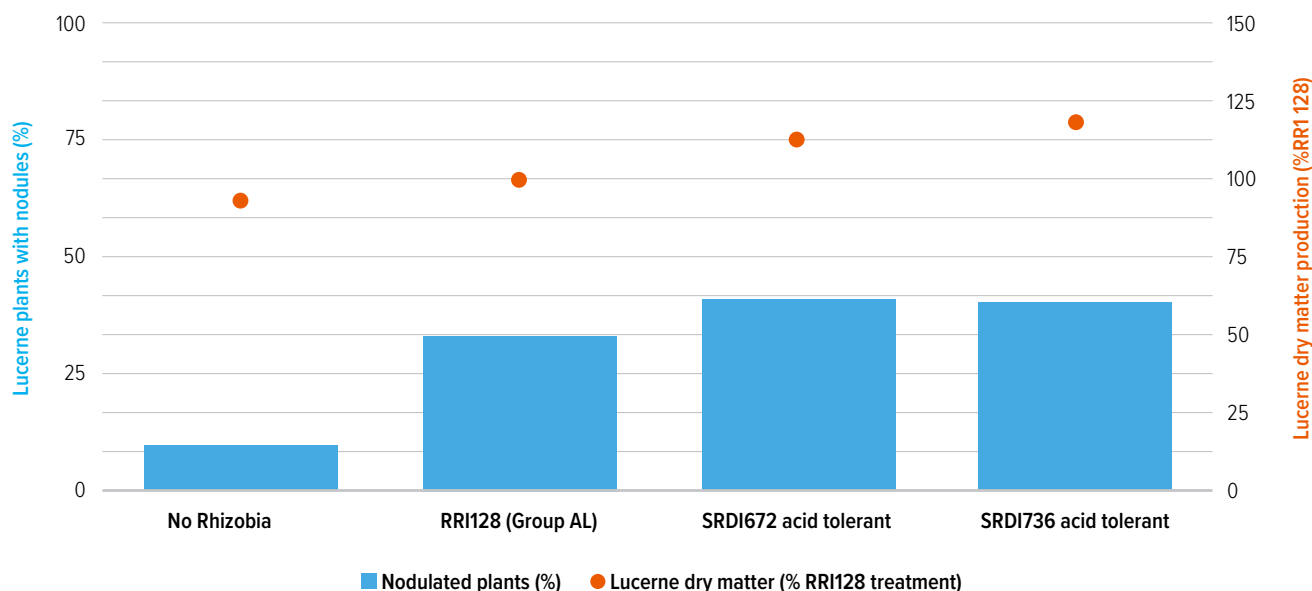
FIGURE 2-21. Rhizobia strain SRDI736 improved lucerne nodulation and dry matter production (mean of 32 assessments) across four field trials ( pH_{Ca} 4.1 to 4.8). SRDI736 is recommended for use with SARDI 7 series 2 lucerne on soils of pH_{Ca} 4.5 to 5.0.
