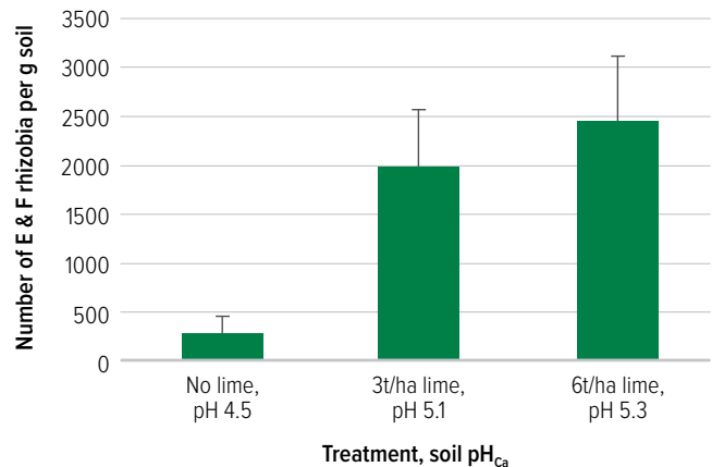
FIGURE 6-8. Effect of lime application in 2018 on soil pH Ca (0 – 10cm) and the number of E and F rhizobia persisting in the soil, when measured in February 2021. Bars indicate standard error.
