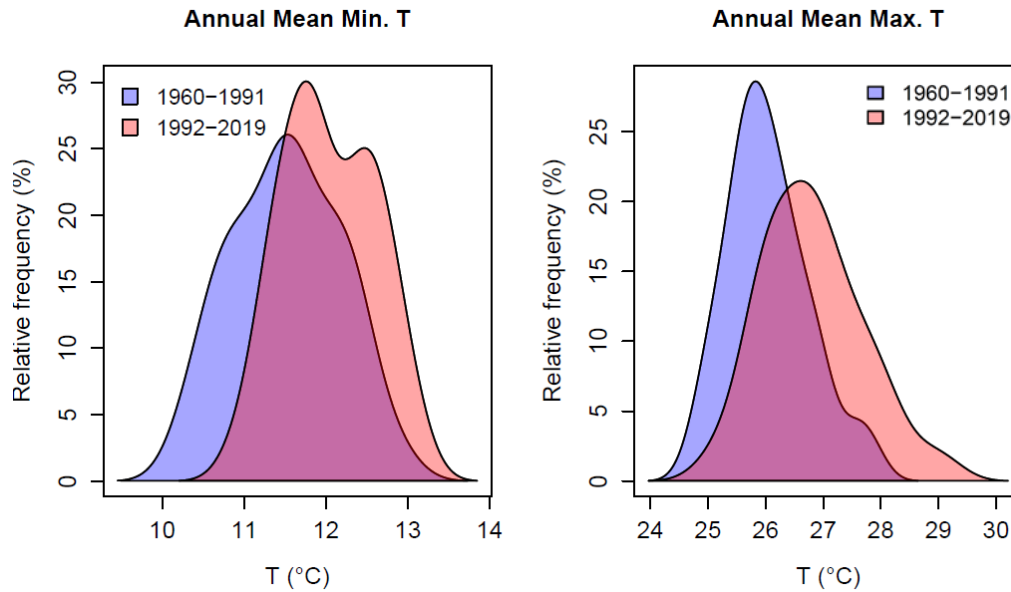
Figure 1. Probability distributions of annual mean maximum temperature (right) and annual mean minimum temperatures (left) for Bellata for two periods, namely 1960 to 1991 and 1992 to 2019.
