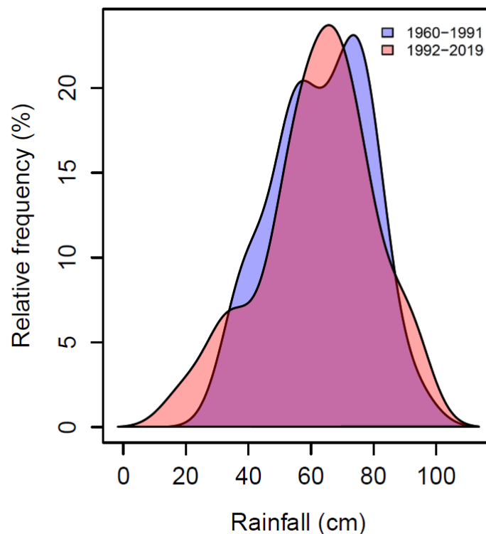
Figure 3. Probability distributions of annual rainfall amounts for Bellata for two periods, namely 1960 to 1991 (blue) and 1992 to 2019 (pink).
