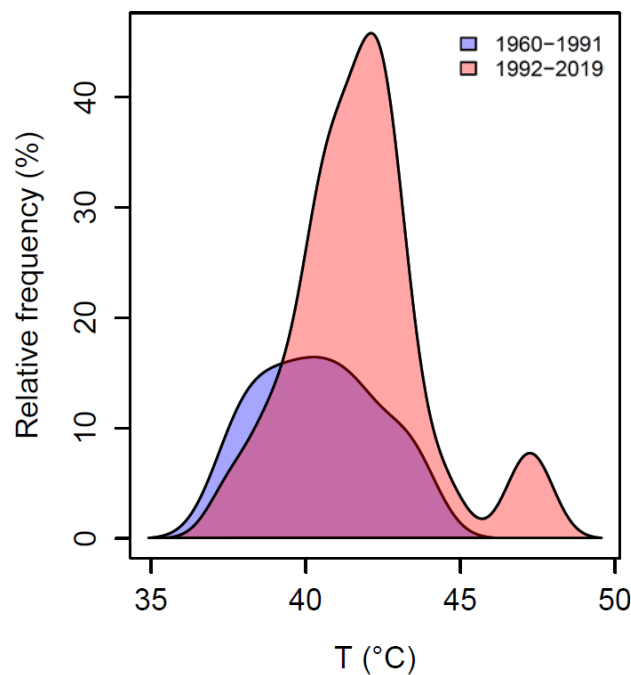
Figure 2. Probability distributions of daily maximum temperature extremes for Bellata for two periods, namely 1960 to 1991 (blue) and 1992 to 2019 (pink).
